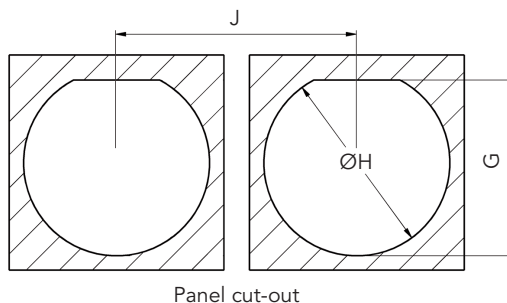
8T7 type Jam nut receptacle with accessories thread
