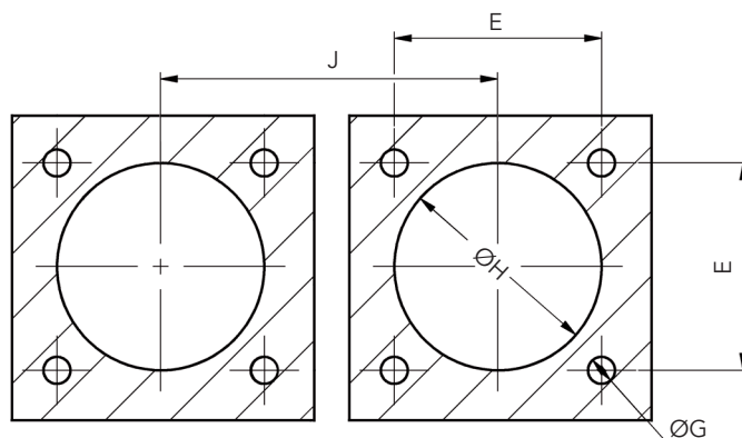
Panel cut-out
