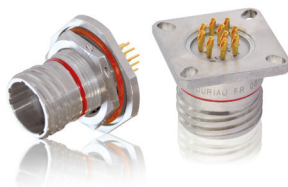
Glass sealed connector see page 137
